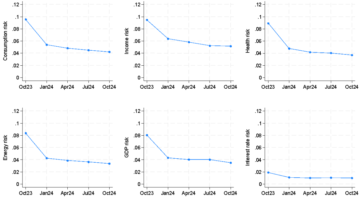
Figure C1. Uncertainty indicators, 2023-24
